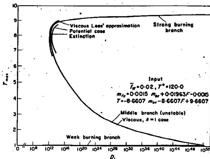
FIG. 6. Plot of T_{\max} vs. D_1 showing ignition and extinction states.
