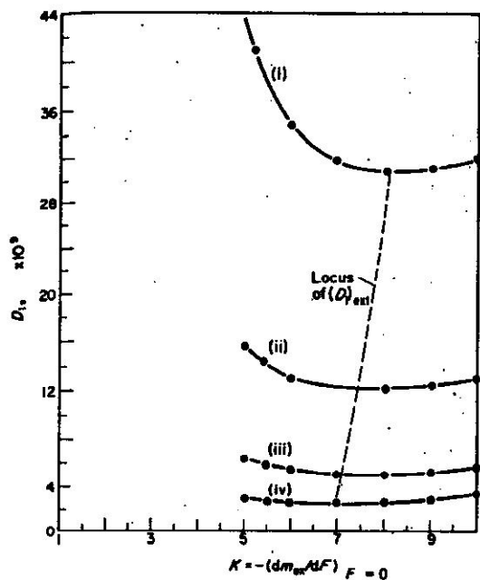
FIG. 10. Effect of the variation of jet temperatures on D_1 ( T_\infty = T_w ). (i) T = 300^\circ\text{K} , T^* = 120 ; (ii) T = 400^\circ\text{K} , T^* = 90 ; (iii) T = 500^\circ\text{K} , T^* = 72 ; (iv) T = 600^\circ\text{K} , T^* = 60 .
