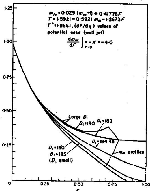
FIG. 3. Variation of oxidant concentration with F ( D_1 varying).
