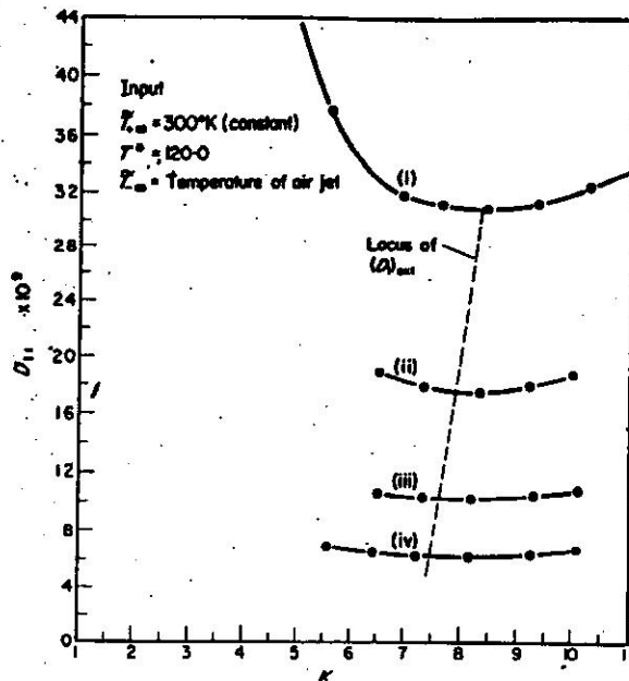
FIG. 11. Variation of Damköhler number with gradient for various air jet temperatures. (i) = 300^\circ\text{K} ; (ii) = 400^\circ\text{K} ; (iii) = 500^\circ\text{K} ; (iv) = 600^\circ\text{K} .
