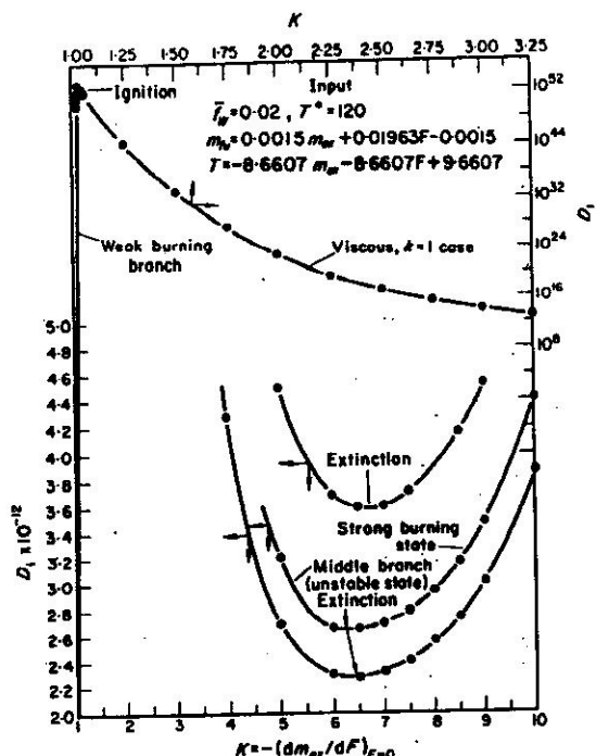
FIG. 5. Plot of D_1 vs. K showing extinction and ignition states.
