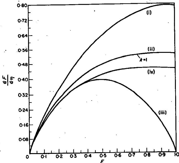
FIG. 2. Plots of dF/d\eta (= F') vs. F . (i) Potential wall-jet: solution of F = \operatorname{erfc}(\eta/\sqrt{2}) ; (ii) Viscous wall-jet: numerical of ff''' + f''' + (1/k+1)(1-f'^2) = 0 , F''' + fF' = 0 ; (iii) Opposed jet: solution of F = \frac{1}{2}[1 + \operatorname{erf}(\eta/\sqrt{2})] ; (iv) Wall-jet: viscous, Lees' approximation: numerical solutions of ff''' + f''' = 0 , F''' + fF' = 0 .
