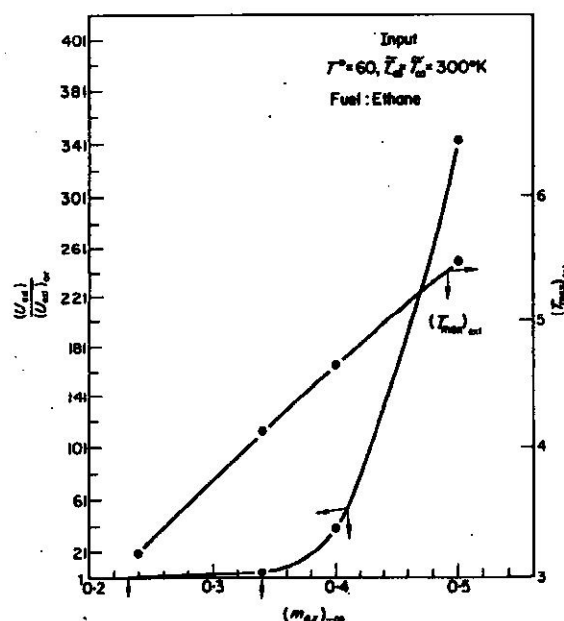
FIG. 9. Effect of variation of oxidant concentration on (U_{\text{ext}}) and (T_{\max})_{\text{ext}} .
