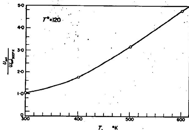
FIG. 12. Variation of extinction speed with temperatures of air jet for the opposed case (hydrogen-air).
