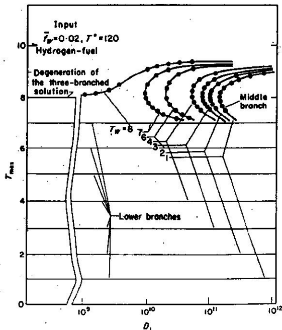
FIG. 8. Variation of T_{\max} with D_1 for various wall temperatures.
