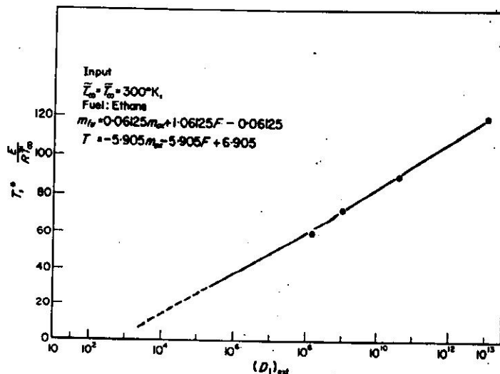
FIG. 13. Effect of variation of activation energy on (D_1)_{ext} .
