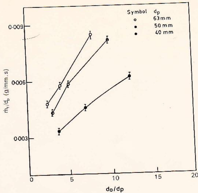
Figure 5. Plot of \dot{m}_f/d_p against d_0/d_p
