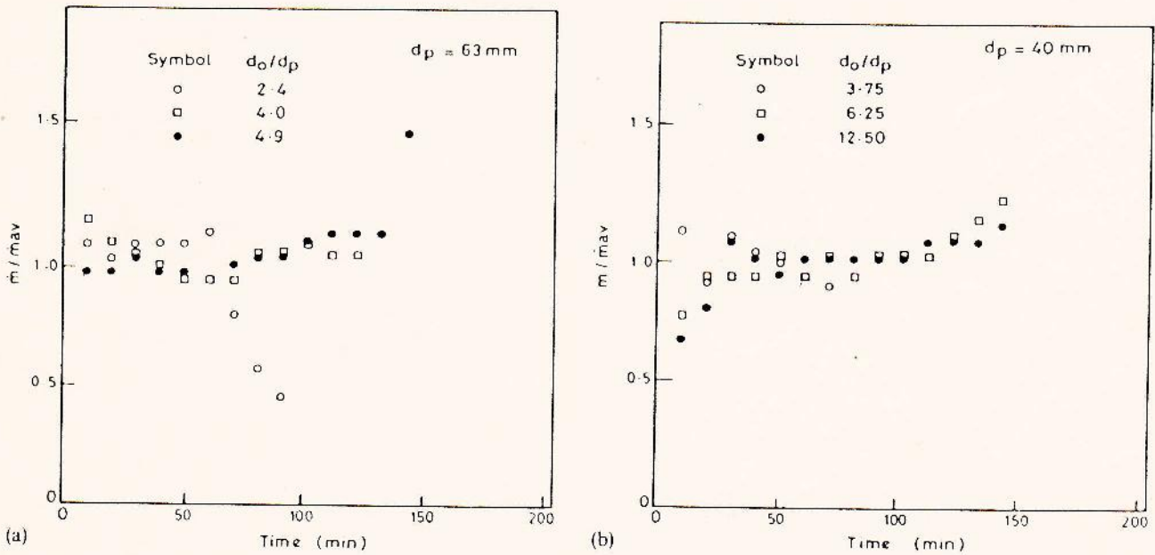
Figure 4. Variation of ratio of fuel mass loss rate to initial mass loss rate with time during operation of stove
