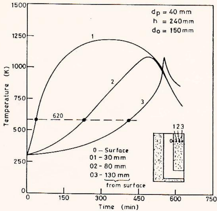
Figure 3. Variation of local temperature at three locations inside fuel block with time for stove in operation
