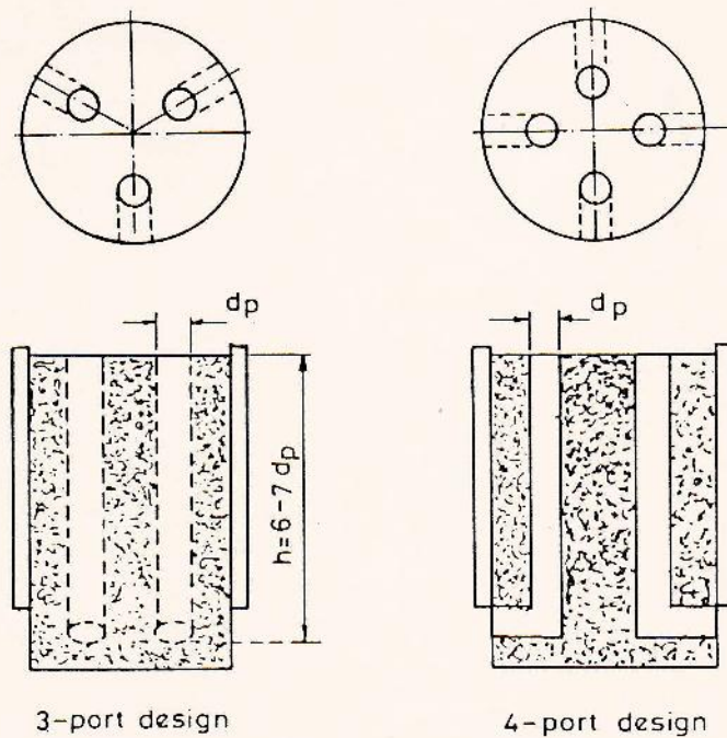
Figure 7. Multiport configurations for stove design
