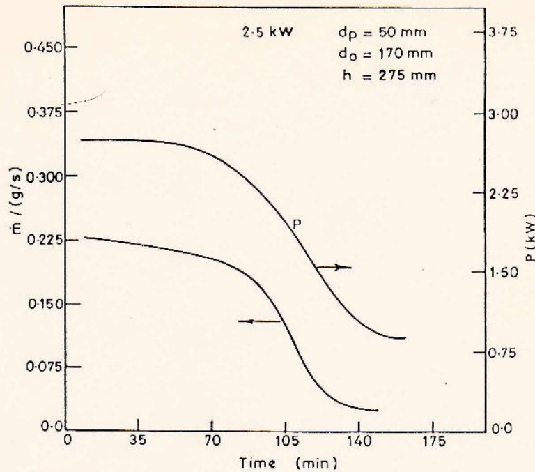
Figure 2. Variation of fuel mass loss rate and estimated power with time in a typical operation
